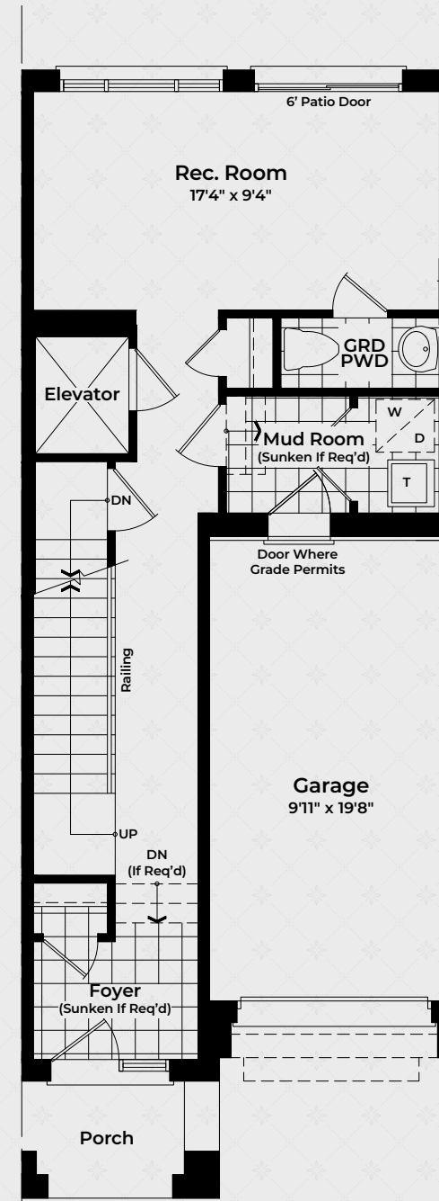
GROUND FLOOR Elev. A W/ Elevator
