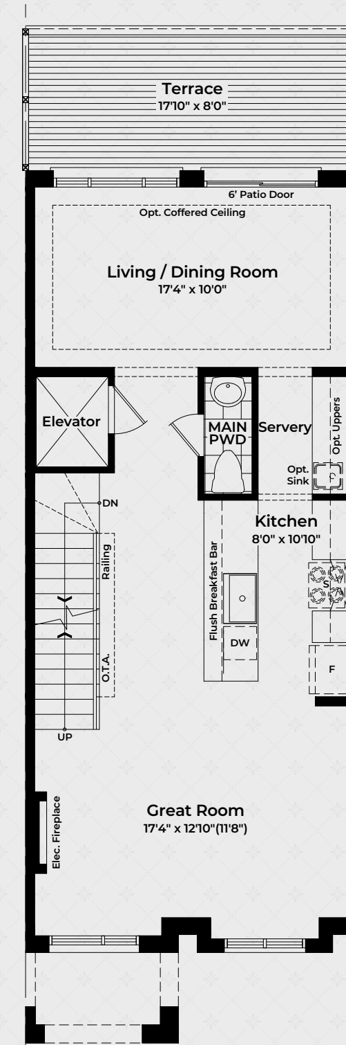
MAIN FLOOR Elev. A W/ Elevator
